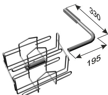
Universal grip
