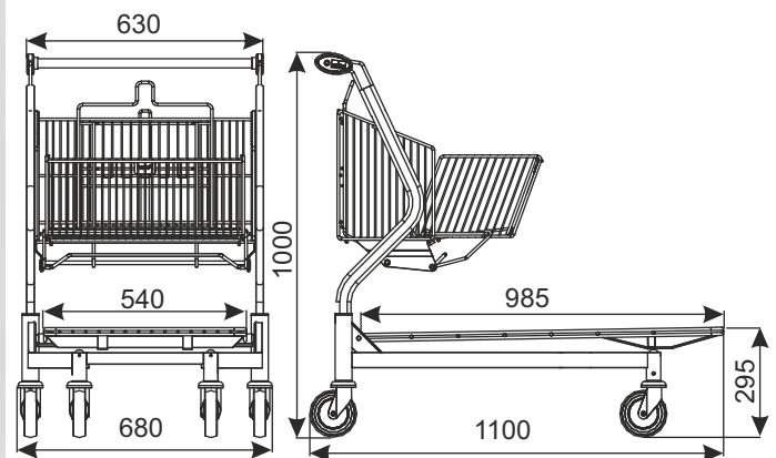
unfolded basket
