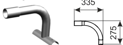
1. Side pipe starting module
