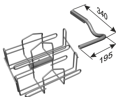
Right grip
